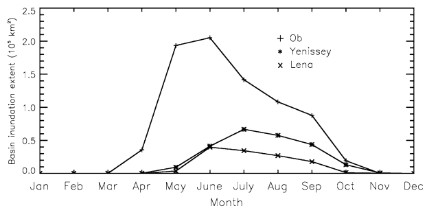
Fig. 2 1993–2000 mean monthly total inundation extent ( \text{km}^2 ) over the three basins
