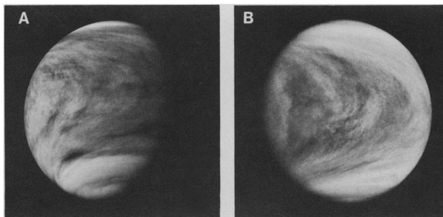
Fig. 2. Images 98 (A) and 291 (B) showing the region near the morning and evening terminators, respectively, during an absence of the large-scale Y feature. These images demonstrate the presence of bow-shaped features as far upstream and downstream of the subsolar point as it is possible to observe. Image (A) resembles the Mariner 10 images except that bow shapes are evident in the morning quadrant and that it is the only image other than 199 (Fig. 1C) among those we have examined to show circumequatorial belts. Image (B) exhibits several bow-shaped features in the afternoon quadrant that form the classical “reverse C” shape observed in low resolution from Earth. When viewed in greater detail, several of the bow shapes appear to be partially composed of “chains” of small polygonal cellular features. Comparisons of these two images illustrate the generally higher contrasts near the evening terminator (B) than near the morning terminator (A), a tendency noted in other such image pairs.
