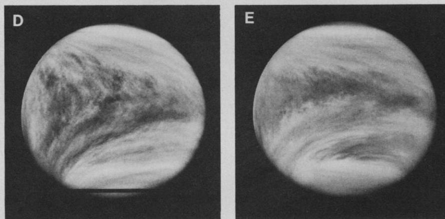
Fig. 1. A sequence of five images illustrating the development and variability of the ultraviolet cloud features over a 6-day period. The first two images, 190 and 194 (A and B), are separated by 1 day and show a feature that with some difficulty may be identified as a dark horizontal Y shape moving into view from the right. The Y appears to be produced by a combination of features, namely (i) a dark equatorial band that is broader in the downstream direction and that joins two dark bands stretching from low to middle latitudes in the downstream direction; (ii) a tilted, bright south polar band and associated bright streaks nearly parallel to the dark bands; and (iii) bow-shaped features often located in the vertex region of the Y. The variation in appearance of each of these features produces the change in the appearance of the Y feature from one recurrence to the next. The relative contrast and shape of the Y in (B) are not symmetric about the equator; such asymmetry is characteristic of the preceding 12 days and similar to that in the Mariner 10 images (5). The next three images—199, 202, and 204 (C to E)—show a very different Y feature moving across the disk. (D) A Y feature that is much more symmetrical and generally broader than the more typical Y 4 days earlier (B). The arms of the Y are formed by several bow-shaped features, which along with the small-scale cellular structure in the center of the disk, give this Y a mottled appearance. The progression in images (C to E) indicates a single Y feature stretching nearly all the way around the planet. Although a similar but shorter Y shape appeared 4 days later, the pattern broke down after that, becoming a more distorted feature as in (B) before disappearing altogether. The region between the bright south polar band and the morning terminator in (A) became considerably brighter as it moved farther onto the disk in (B), illustrating a general tendency for low contrast near the morning terminator. Image (C) shows a number of faint circumequatorial belts identified by Mariner 10 but seen only rarely in the current images. The south polar band in (E) exhibits a “kink” near its left-hand extremity, and the northern edge of the band is disrupted by a series of dark tilted streaks, a condition observed on many occasions.
