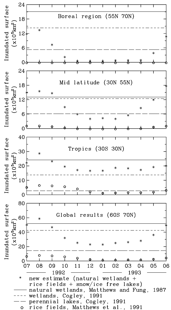
Figure 4. Seasonal variations of the inundated areas globally and by latitude zones. Static estimates from Matthews et al. and Cogley are also indicated.
