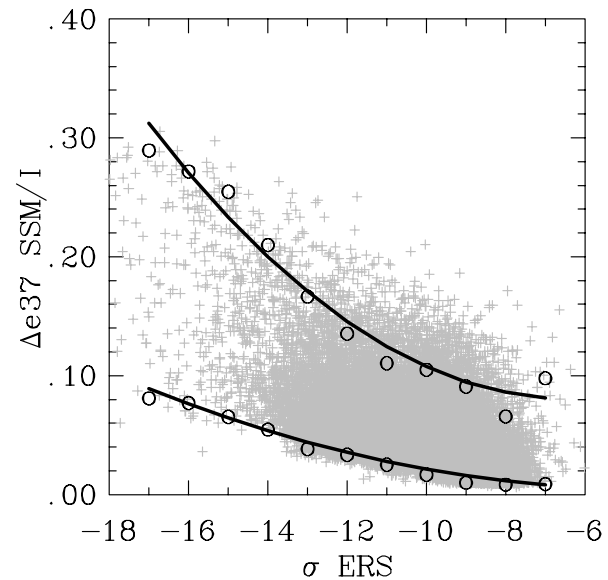
Figure 2. Active microwave \sigma versus passive microwave \Delta e_{37} for pixels classified as inundated. For each 1 dB range of \sigma , mean \Delta e_{37} are calculated for the 10 % lowest and highest \Delta e_{37} and are plotted.
