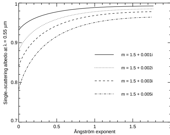
Fig. 3. Aerosol single-scattering albedo versus Ångström exponent for \text{Re}(m)=1.5 and four increasing values of \text{Im}(m) .
