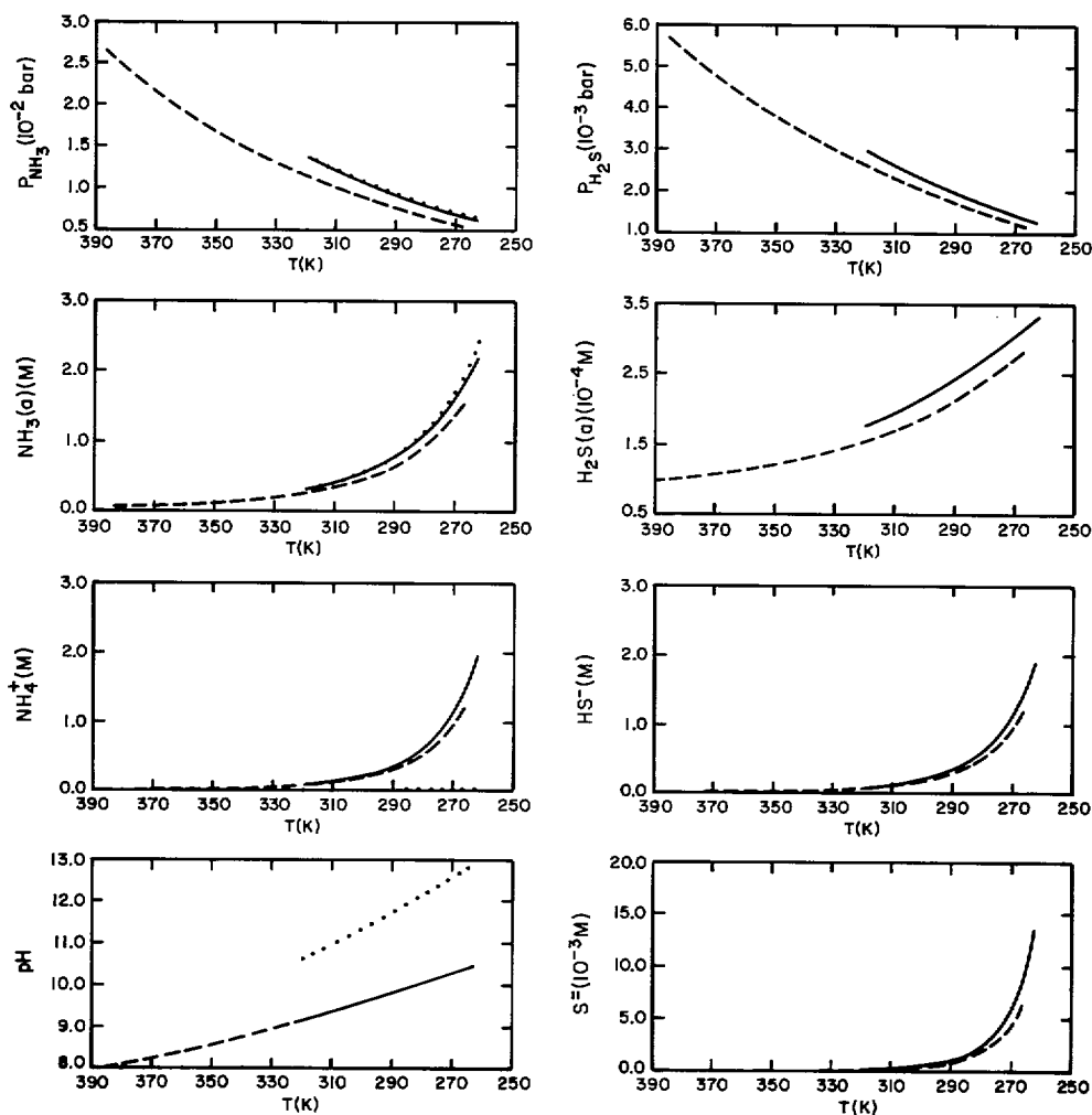
FIG. 1.—Properties of the water cloud chemistry on Uranus as a function of temperature. A comparison is made between the complete aqueous chemistry determined by the three component system, NH 3 -H 2 O-H 2 S (solid lines), by the chemistry without H 2 S (dotted lines), and by the chemistry with a 10 × solar enhancement of H 2 O (dashed lines). The partial pressures of NH 3 and H 2 S in the atmosphere are shown in the top panels; the molar concentrations of the dissolved (aqueous) gases in the cloud drops, in the panels immediately below. Ionic concentrations of NH 4 + , HS - , and S = , as well as pH are also included.
